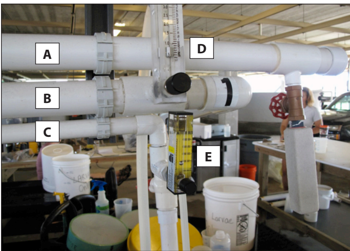
Figure 4. System manifolds and flow meters, including: A = air manifold (1.5-inch-diameter PVC pipe); B = seawater manifold (1.5-inch-diameter PVC pipe); C = algal manifold ( \frac{3}{4} -inch-diameter PVC pipe); D = seawater flow meter; and E = algal flow meter. Tubing is used to deliver seawater and algae from the flow meters to the tank surface.
