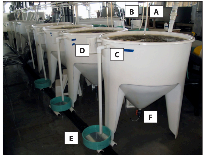
Figure 1. An eight (400-L) tank flow-through system. Each tank includes: A = incoming seawater tube; B = incoming algal tube; C = seawater discharge; D = 6-inch-diameter overflow trap; E = 12-inch-diameter floor trap; and F = incoming air and drain valve.
